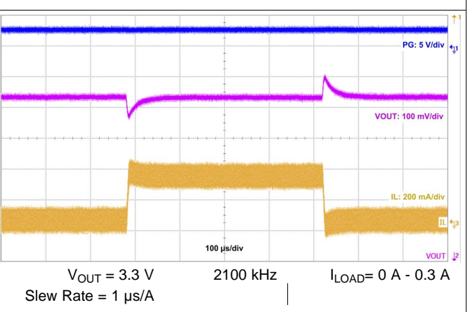
Figure 49. Load Transient
