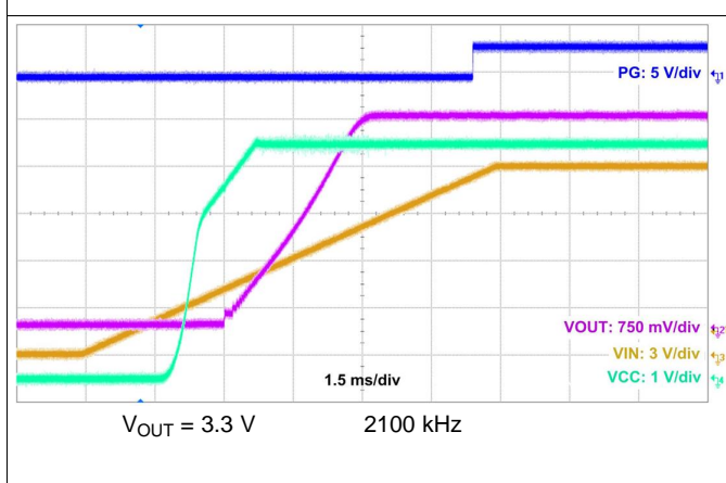
Figure 48. Start-Up Waveform
