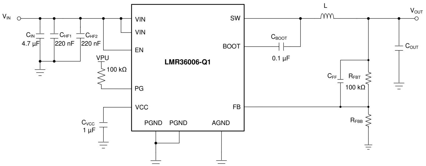
Figure 18. Example Applications Circuit (Adjustable Output)
