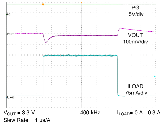
Figure 33. Load Transient
