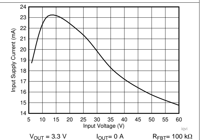
Figure 47. Input Supply Current
