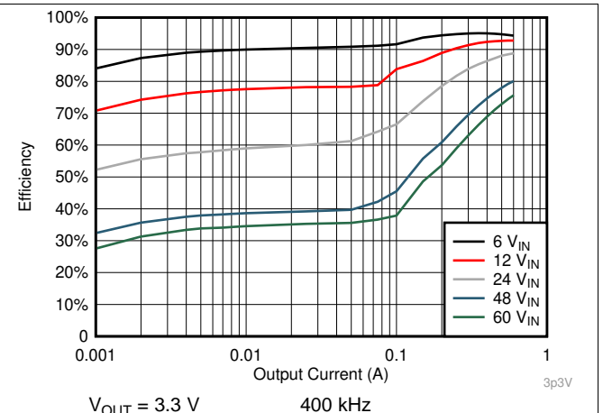
Figure 23. Efficiency
