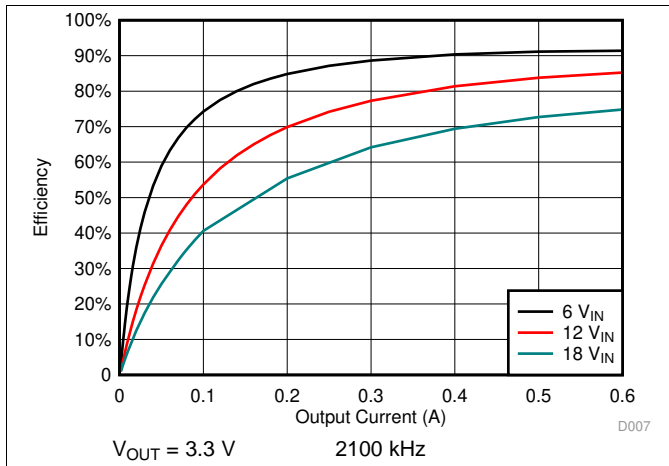
Figure 44. Efficiency
