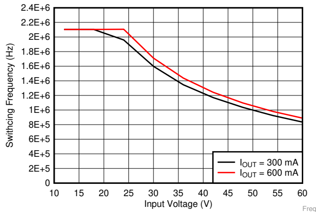
Figure 17. Switching Frequency vs Input Voltage V OUT = 3.3 V
