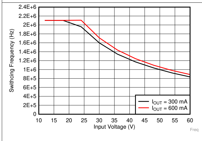
Figure 46. Switching Frequency vs Input Voltage
