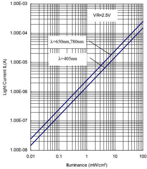
Relative Sensitivity vs. Illuminance (Ta=25°C)
