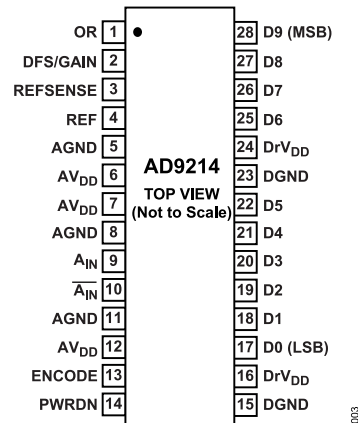
Figure 3. Pin Configuration
