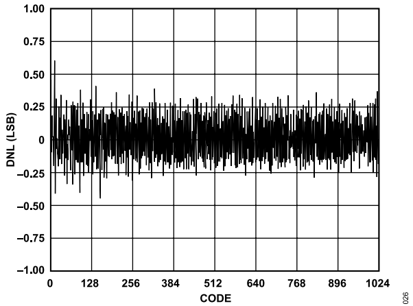
Figure 21. DNL @ 80 MSPS
