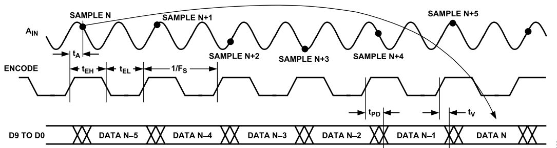
Figure 2. Timing Diagram
