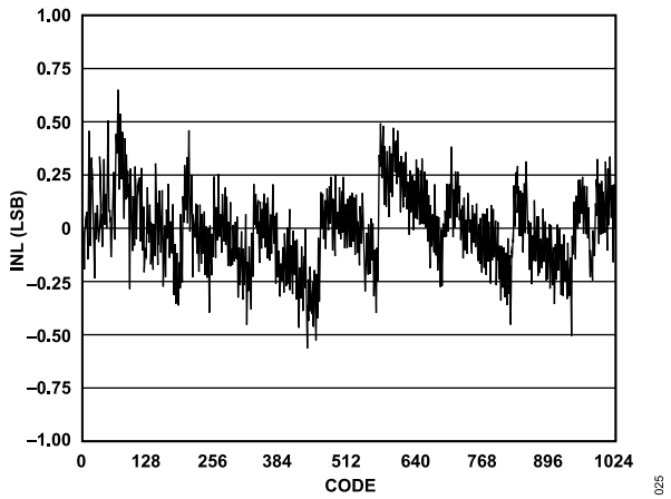
Figure 20. INL @ 80 MSPS
