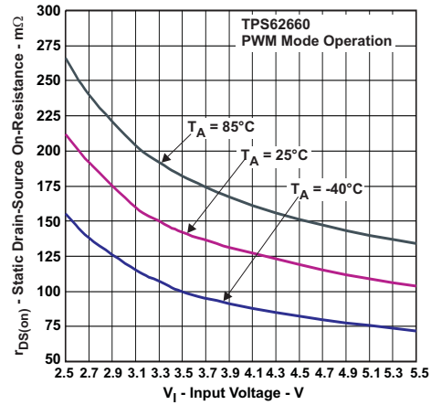
Figure 33. N-Channel r_{DS(ON)} vs Input Voltage
