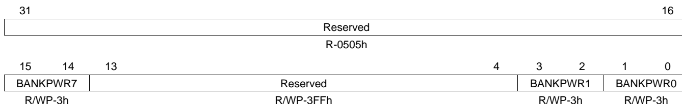
Figure 5-22. Flash Bank Fallback Power Register (FBFALLBACK) [offset = 40h]
