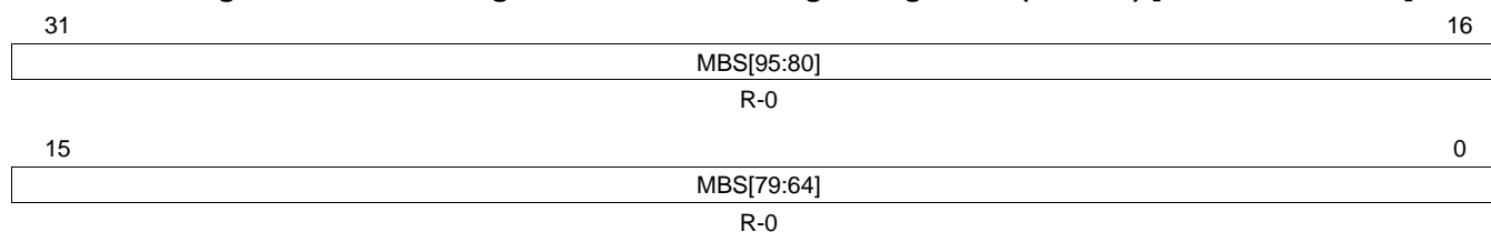
Figure 23-169. Message Buffer Status Changed Register 3 (MBSC3) [offset_CC = 348h]
