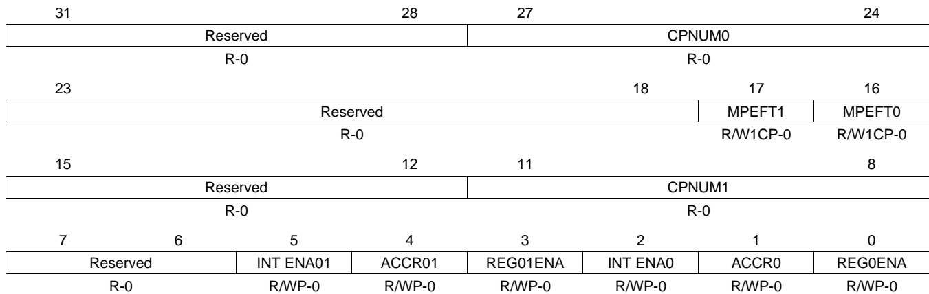
Figure 21-39. Memory Protection Control and Status Register (HTU MPCS) [offset = 70h]
