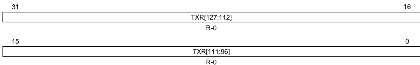
Figure 23-162. Transmission Request Register 4 (TXRQ4) [offset_CC = 32Ch]
