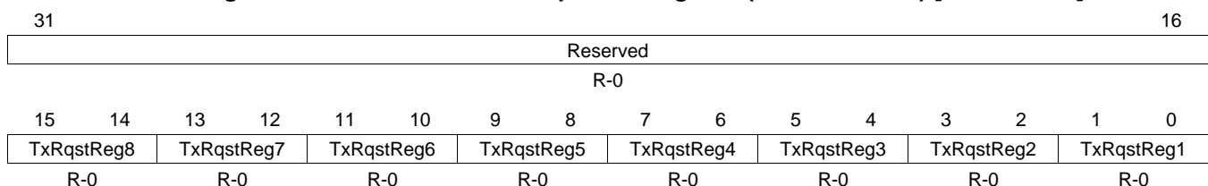
Figure 24-28. Transmission Request X Register (DCAN TXRQ X) [offset = 84h]
