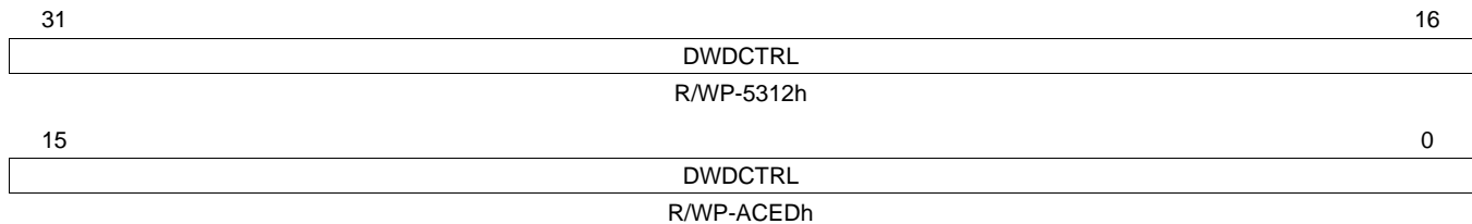
Figure 13-39. Digital Watchdog Control Register (RTIDWCTRL) [offset = 90h]
