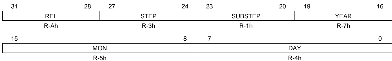
Figure 24-26. Core Release Register (DCAN REL) [offset = 20h]
