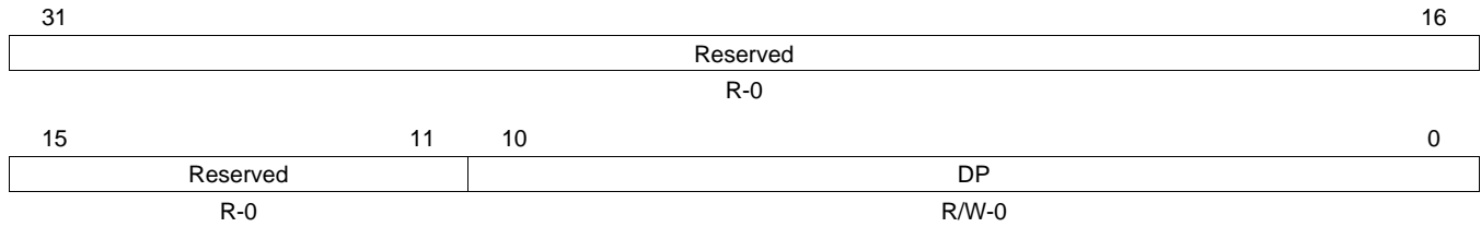
Figure 23-176. Write Header Section Register 3 (WRHS3) [offset_CC = 508h]
