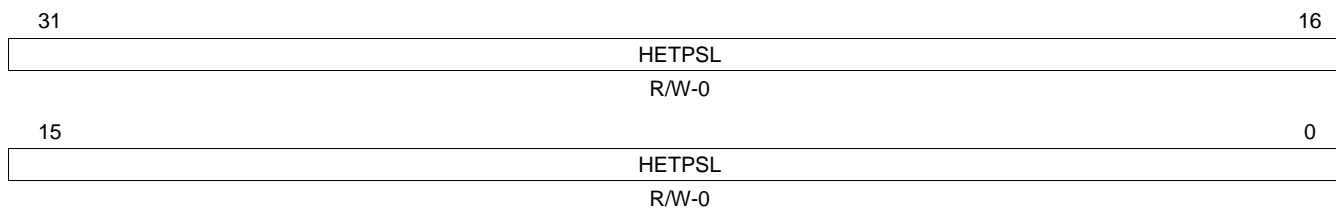
Figure 20-80. N2HET Pull Select Register (HETPSL)
