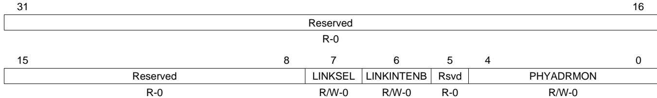
Figure 29-41. MDIO User PHY Select Register 1 (USERPHYSEL1)
