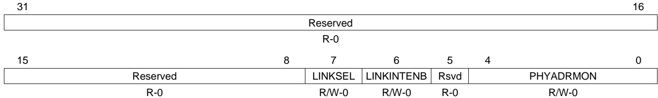
Figure 29-39. MDIO User PHY Select Register 0 (USERPHYSEL0)
