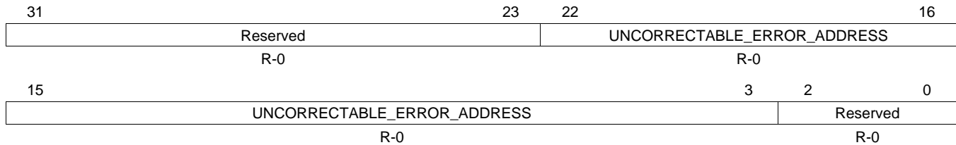
Figure 6-9. TCRAM Module Uncorrectable Error Address Register (RAMUERRADDR) [offset = 1Ch]
