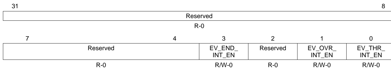
Figure 19-31. ADC Event Group Interrupt Enable Control Register (ADEVINTENA) [offset = 28h]
