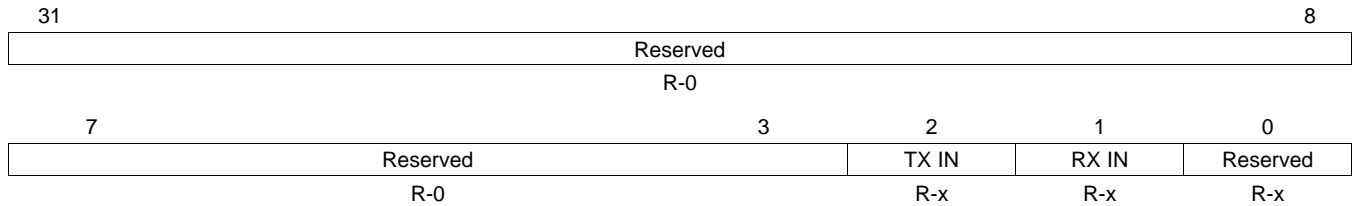
Figure 26-44. SCI Pin I/O Control Register 2 (SCIPIO2) [offset = 44h]
