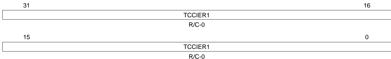
Figure 23-96. Transfer to Communication Controller Interrupt Enable Reset 1 (TCCIER1) [offset_TU = 124h]
