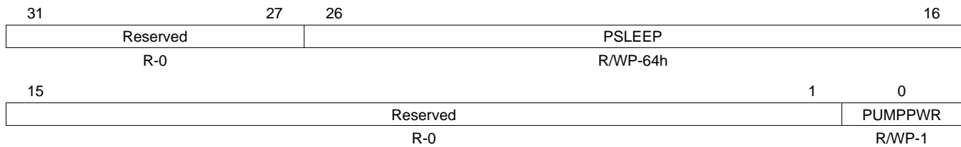
Figure 5-24. Flash Pump Access Control Register 1 (FPAC1) [offset = 48h]
