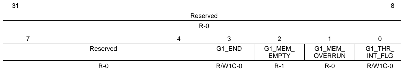
Figure 19-35. ADC Group1 Interrupt Flag Register (ADG1INTFLG) [offset = 38h]
