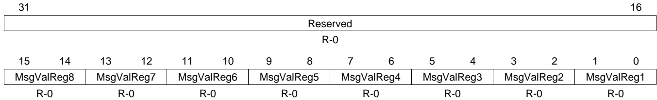
Figure 24-43. Message Valid X Register (DCAN MSGVAL X) [offset = C0h]
