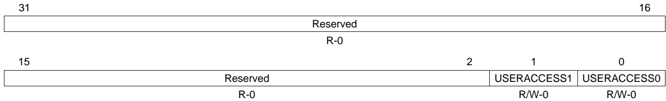
Figure 29-37. MDIO User Command Complete Interrupt Mask Clear Register (USERINTMASKCLEAR)
