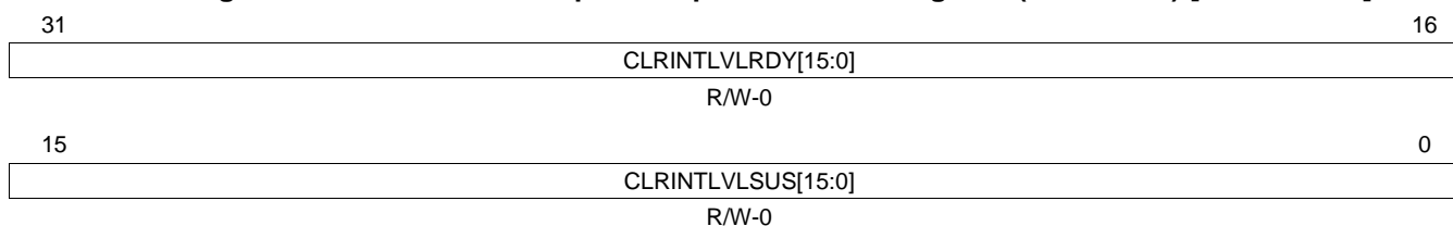
Figure 25-59. Transfer Group Interrupt Level Clear Register (TGITLVCR) [offset = 80h]
