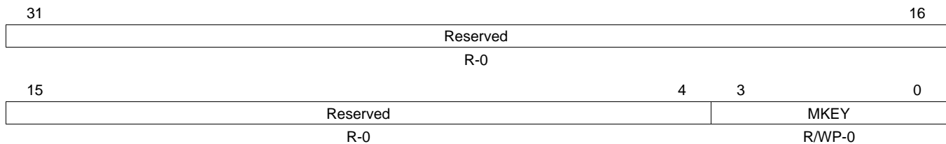
Figure 3-17. PSCON Diagnostic Compare Key Register (PRCKEYREG) [offset = ACh]
