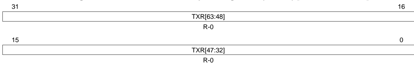
Figure 23-160. Transmission Request Register 2 (TXRQ2) [offset_CC = 324h]
