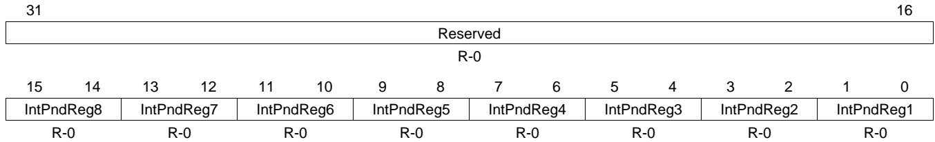
Figure 24-38. Interrupt Pending X Register (DCAN INTPND X) [offset = ACh]
