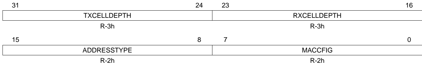
Figure 29-74. MAC Configuration Register (MACCONFIG)
