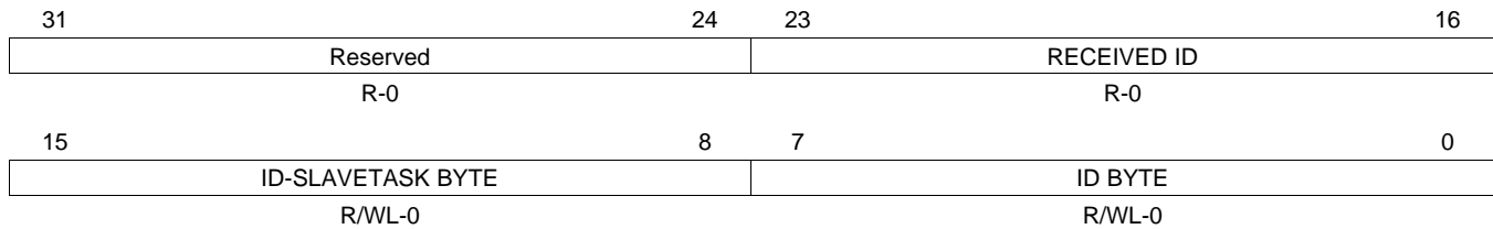
Figure 26-55. LIN Identification Register (LINID) [offset = 70h]
