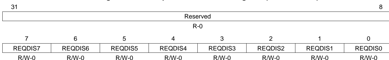
Figure 20-71. Request Enable Clear Register (HETREQENC)
