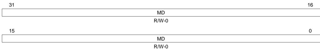
Figure 23-179. Read Data Section Registers (RDDSn) [offset_CC = 600h-6FCh]
