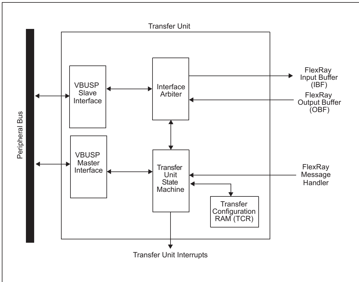
Figure 23-3. Transfer Unit
