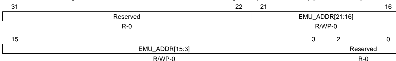
Figure 5-31. EEPROM Emulation Address Register (FEMU_ADDR) [offset = 68h]
