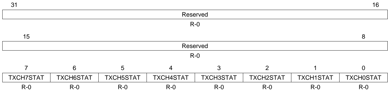
Figure 29-24. EMAC Control Module Transmit Interrupt Status Register (C0TXSTAT)
