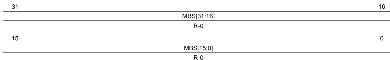
Figure 23-167. Message Buffer Status Changed Register 1 (MBSC1) [offset_CC = 340h]
