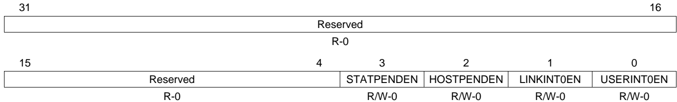
Figure 29-21. EMAC Control Module Miscellaneous Interrupt Enable Register (C0MISCEN)
