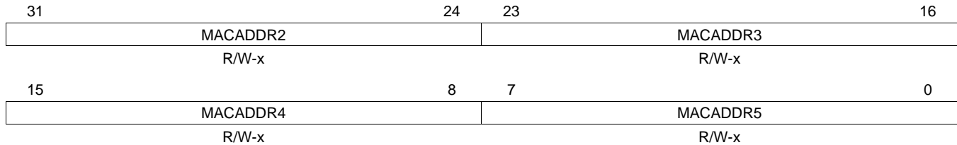
Figure 29-85. MAC Address High Bytes Register (MACADDRHI)
