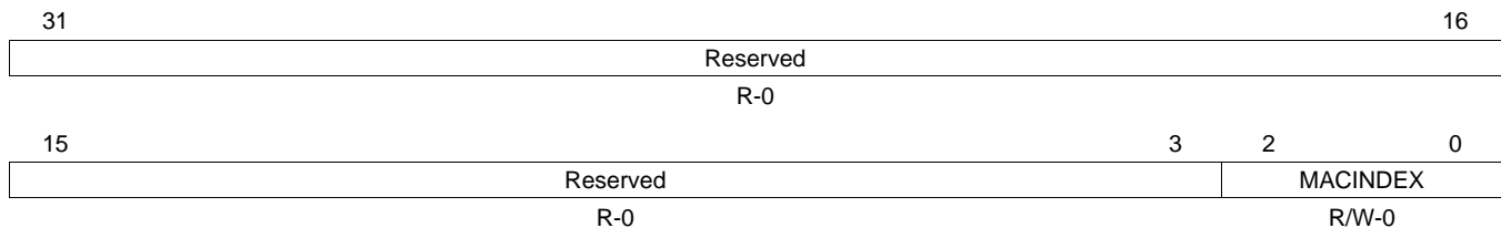
Figure 29-86. MAC Index Register (MACINDEX)
