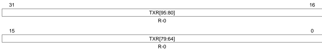
Figure 23-161. Transmission Request Register 3 (TXRQ3) [offset_CC = 328h]
