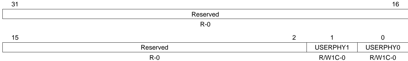
Figure 29-33. MDIO Link Status Change Interrupt (Masked) Register (LINKINTMASKED)
