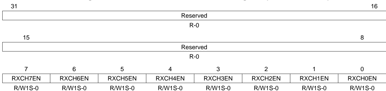
Figure 29-63. Receive Unicast Enable Set Register (RXUNICASTSET)
