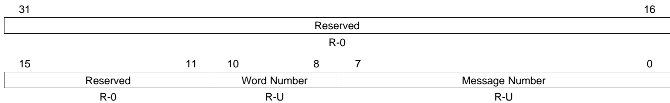
Figure 24-25. Parity Error Code Register (DCAN PERR) [offset = 1Ch]
