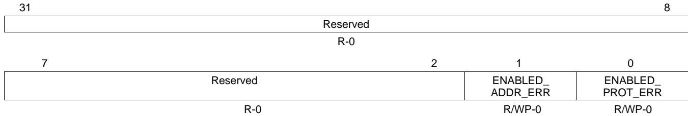
Figure 4-9. ERR_ENABLED_STATUS_REG: Error Enabled Status / Clear Register (Address = FFFF0AE4h)
