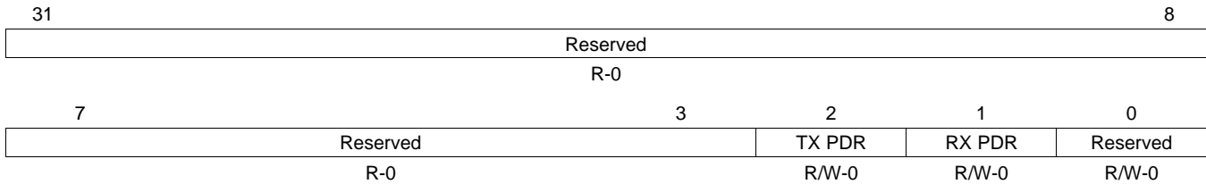
Figure 27-28. SCI Pin I/O Control Register 6 (SCIPIO6) [offset = 54h]
