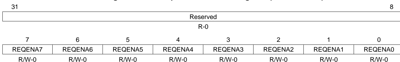
Figure 20-70. Request Enable Set Register (HETREQENS)
