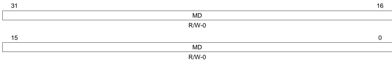
Figure 23-173. Write Data Section Registers (WRDSn) [offset_CC = 400h-4FCh]
