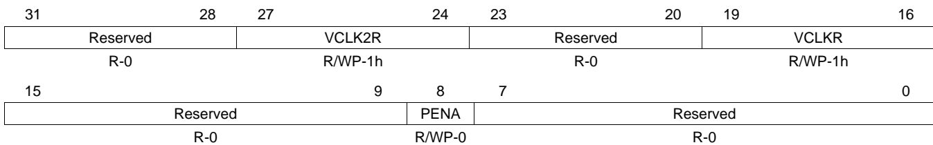
Figure 2-49. Clock Control Register (CLKCNTL) [offset = D0h]
