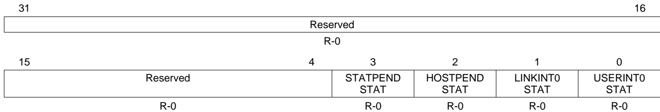
Figure 29-25. EMAC Control Module Miscellaneous Interrupt Status Register (C0MISCSTAT)
