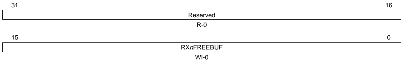
Figure 29-69. Receive Channel n Free Buffer Count Register (RX n FREEBUFFER)
