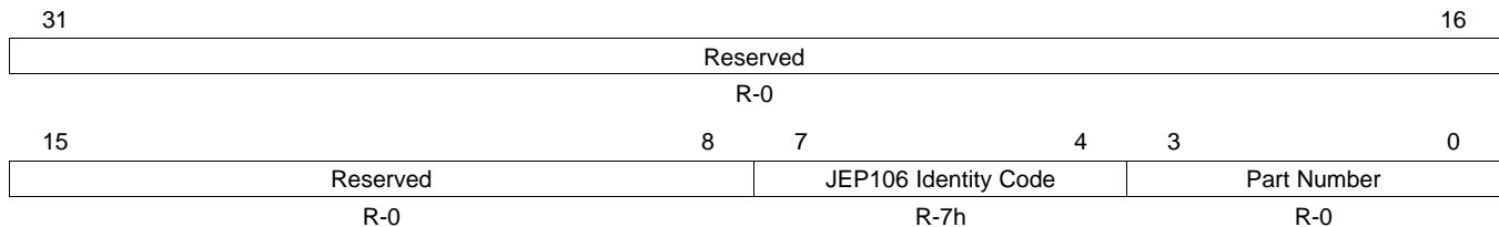
Figure 18-23. POM Peripheral ID 1 Register (POMPERIPHERALID1) [address = FFA0 4FE4]
