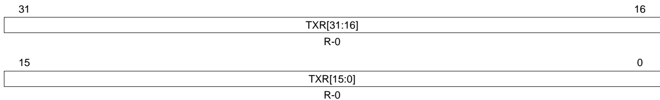
Figure 23-159. Transmission Request Register 1 (TXRQ1) [offset_CC = 320h]
