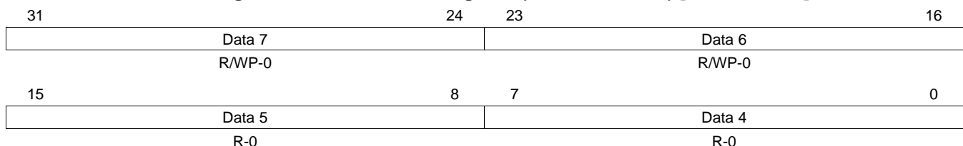
Figure 24-69. IF3 Data B Register (DCAN IF3DATB) [offset = 154h]
