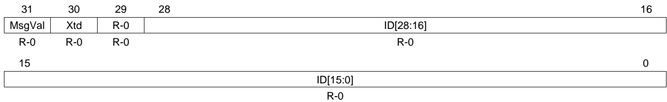
Figure 24-66. IF3 Arbitration Register (DCAN IF3ARB) [offset = 148h]
