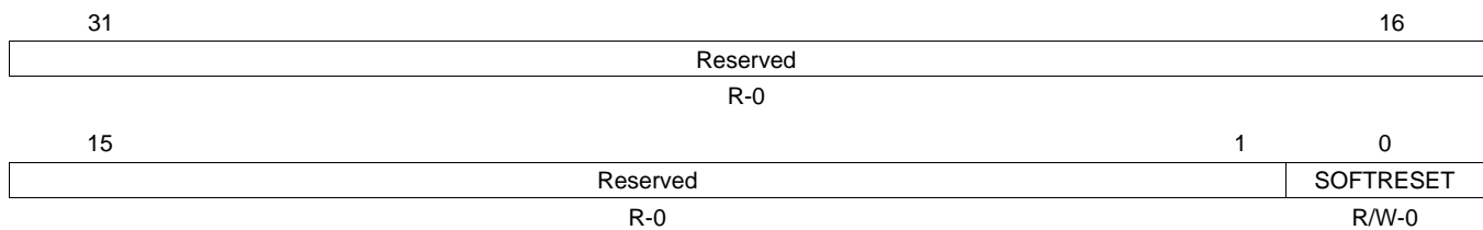
Figure 29-75. Soft Reset Register (SOFTRESET)
